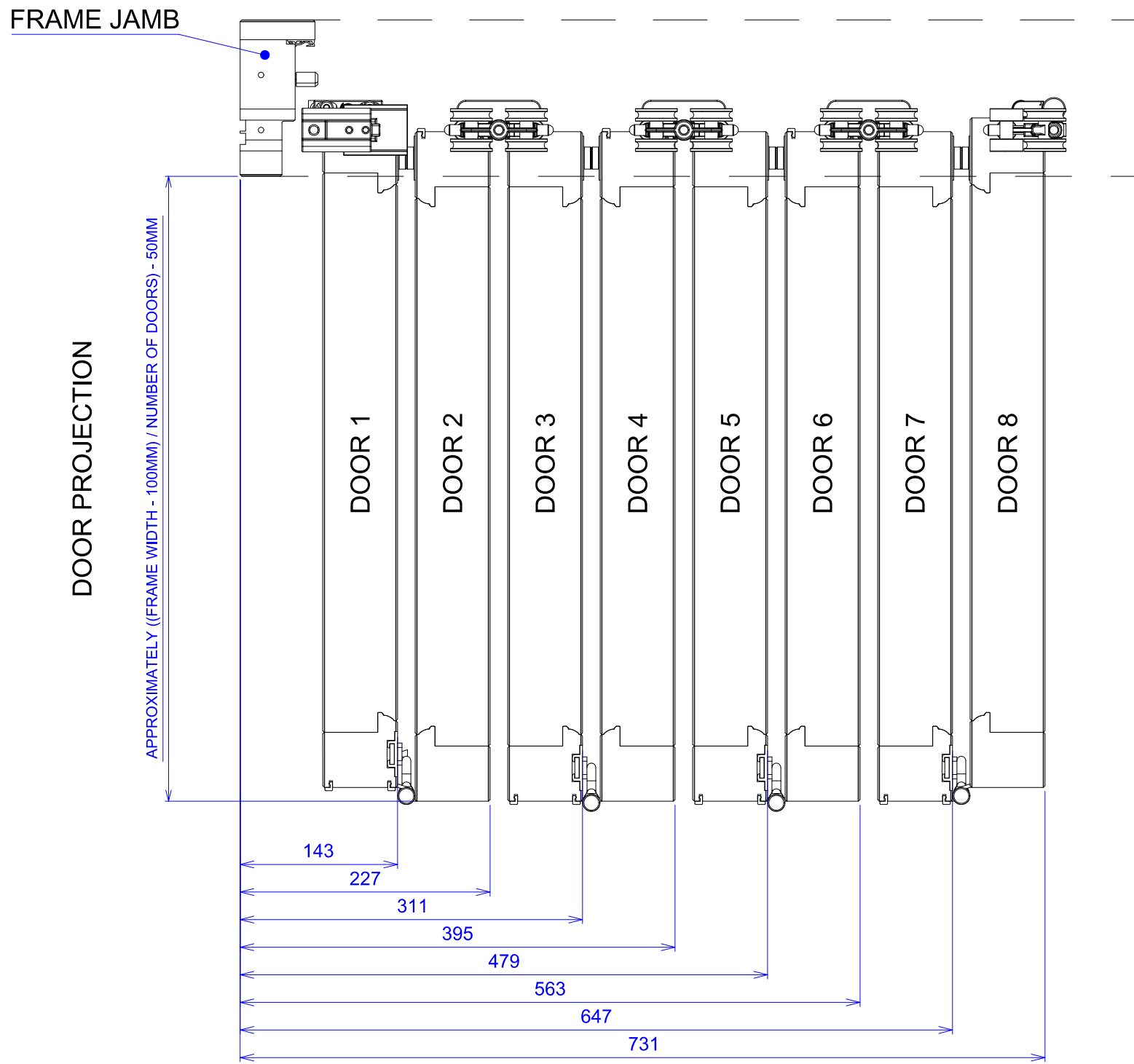
DOOR STACK WIDTHS WHEN FULLY OPEN (JAMB WIDTH - 9MM) + (NUMBER OF DOORS X 84MM)
